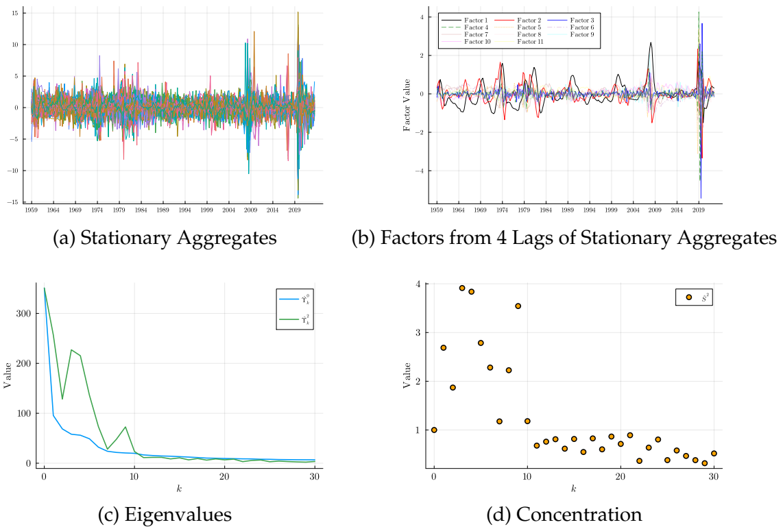
Figure 14: Eigenvalue Analysis of Aggregates
