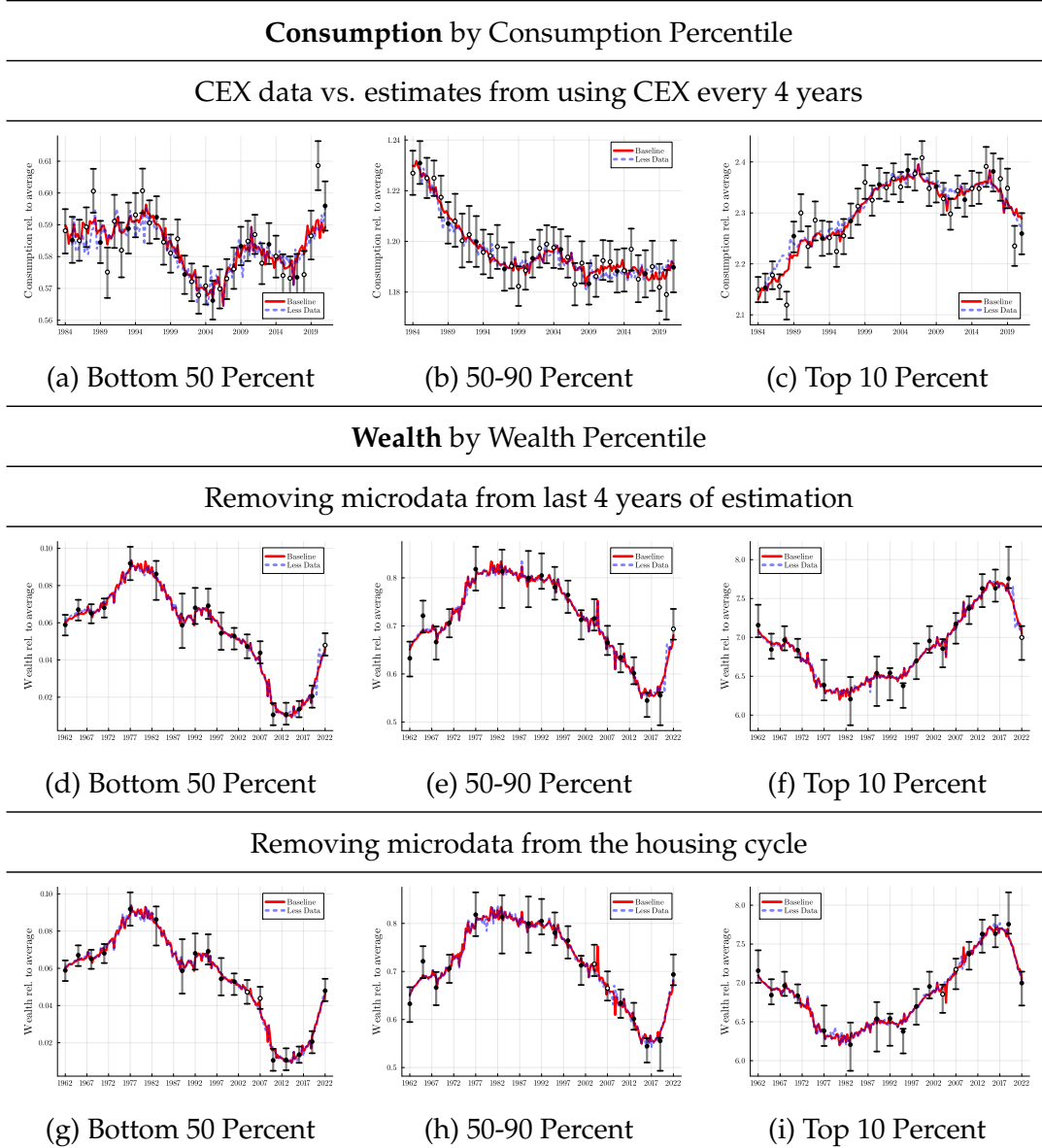
Figure 7: Predictability of Distributional Data (Re-estimating the Model)
