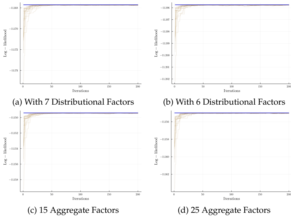
Figure 13: Hyperparameter Convergence: Different Factor Structures
